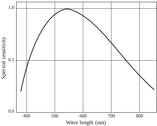
CCD Spectral Responsive Characteristics
